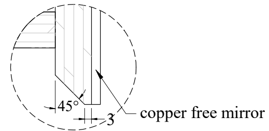
Detail 'X'
