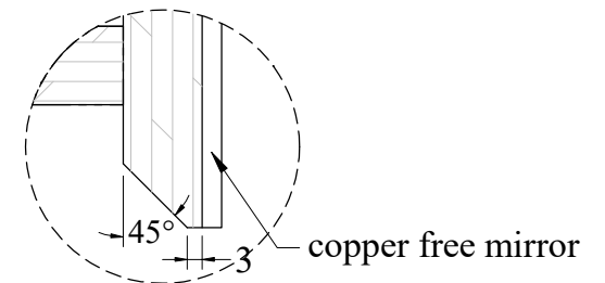
Detail 'X'
