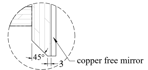
Detail 'X'
